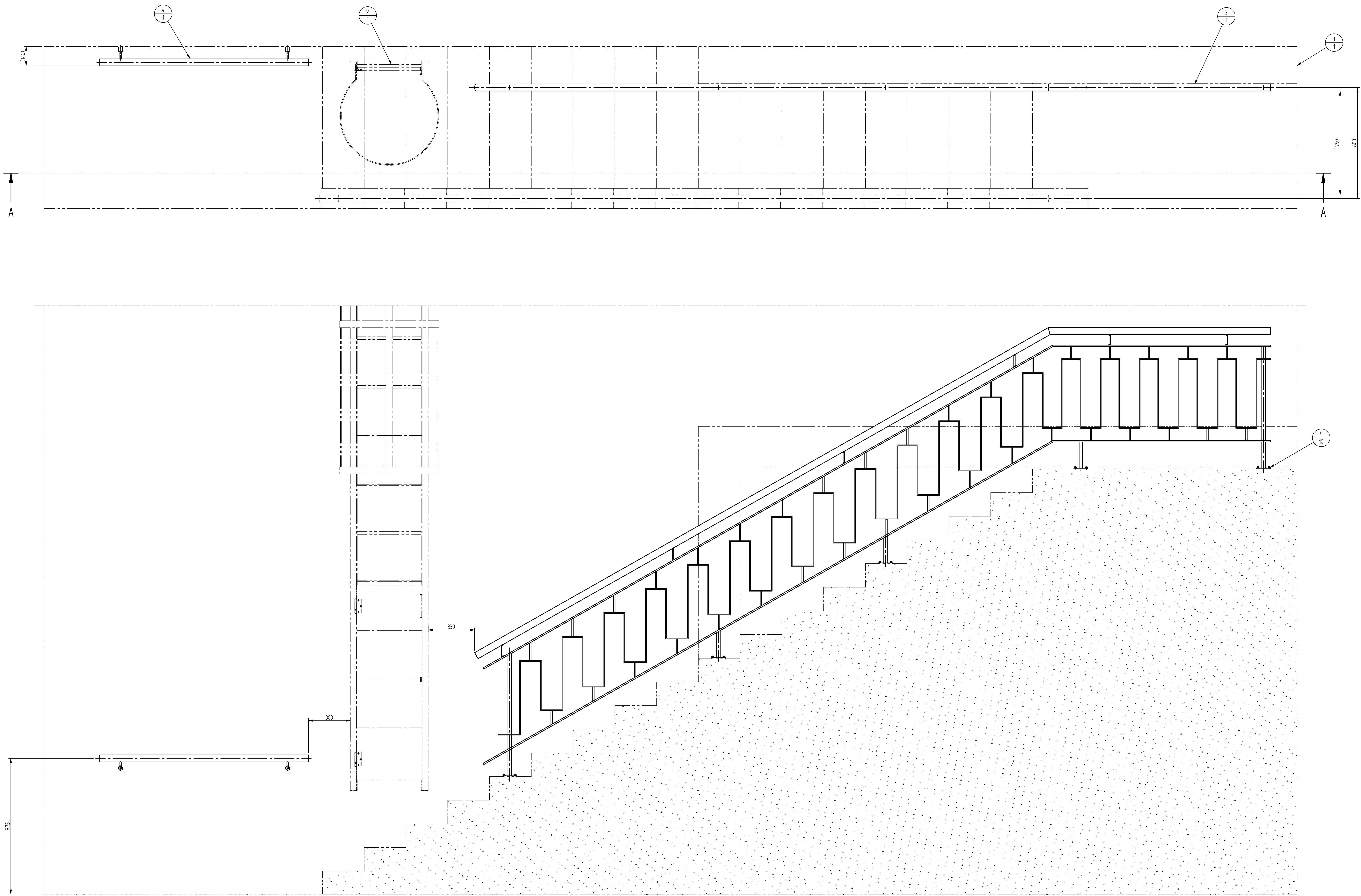
SECTION A-A (EXISTING HANDRAIL HOLDER OMITTED FOR CLARITY.)
