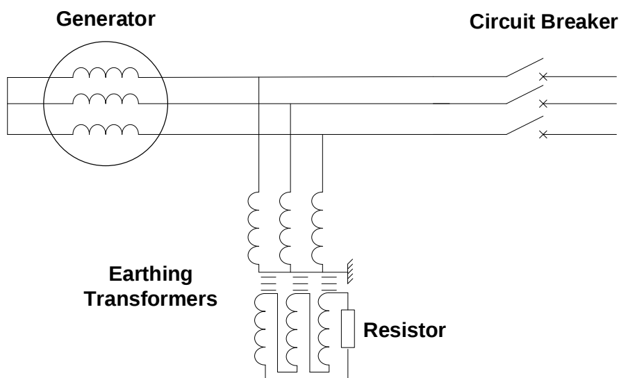
Figure 4: Generator Earthing
