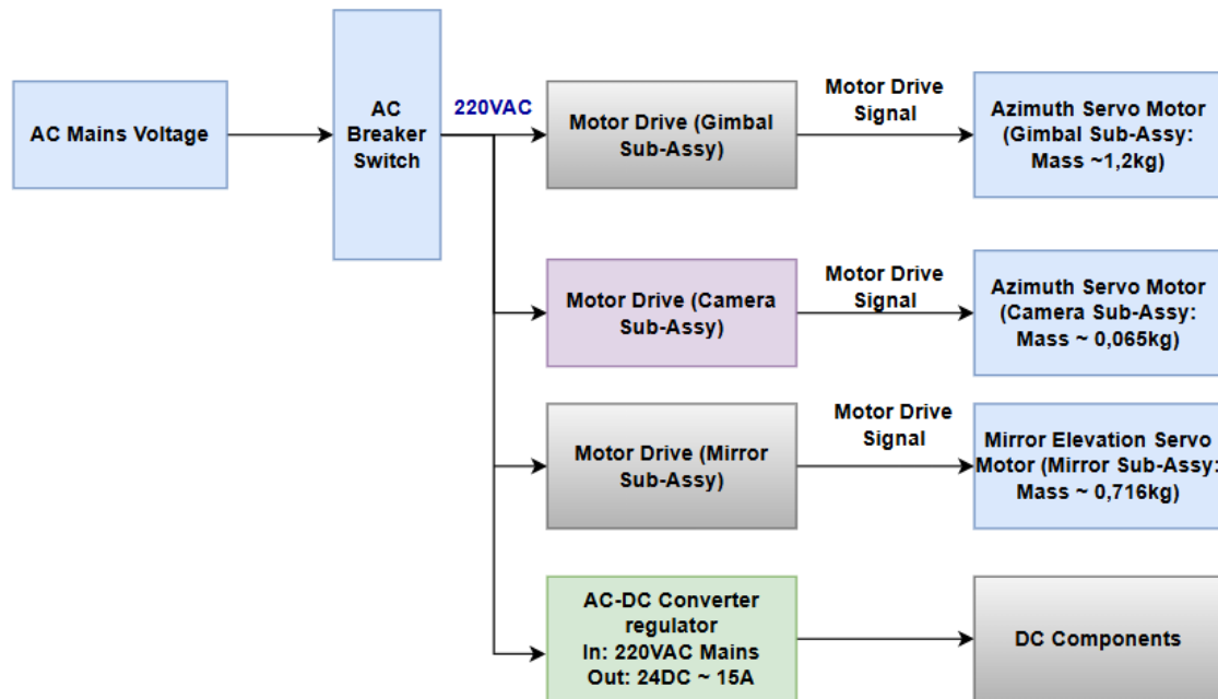
Figure 1: High-Level System Block Diagram
