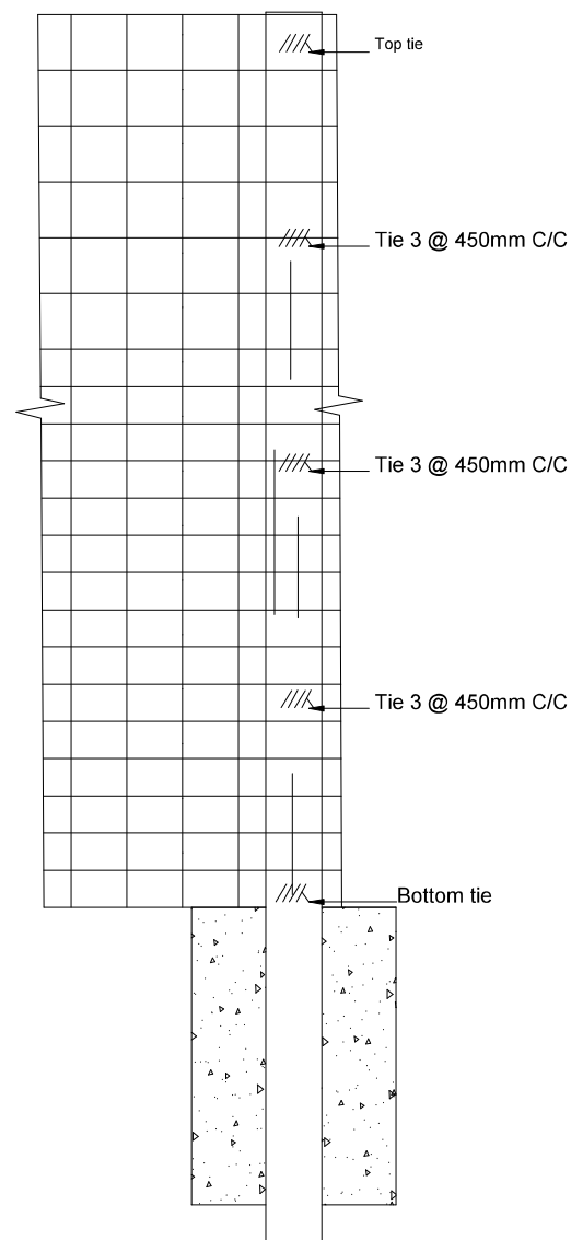
DETAIL A: TYING WOODEN POSTS WITH WIRE
