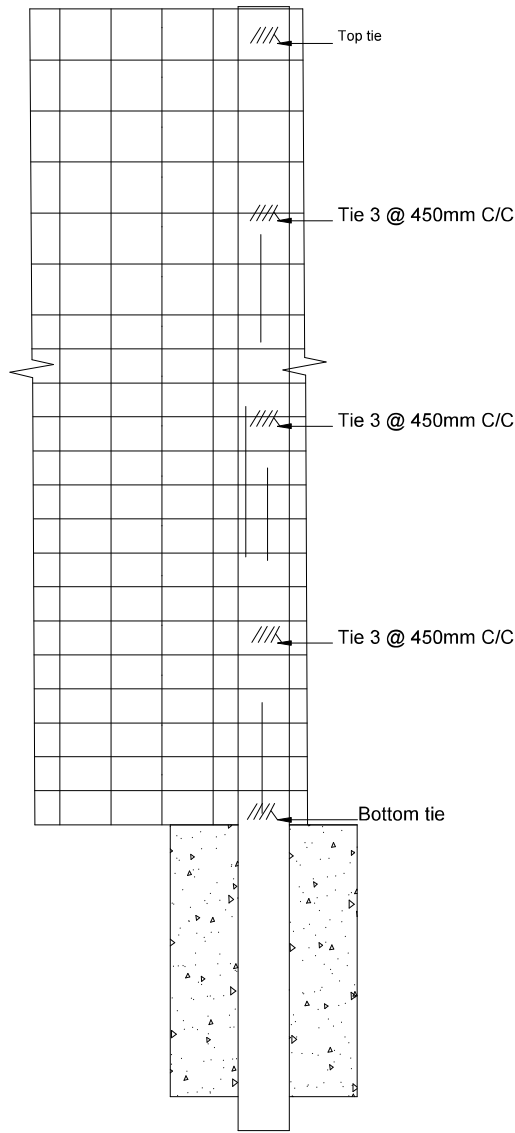
DETAIL A: TYING STEEL TUBULAR POST WITH WIRE
