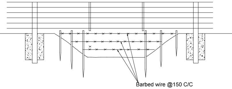
BARBED WIRE ACCROSS THE CHANNEL OR TRENCHES
