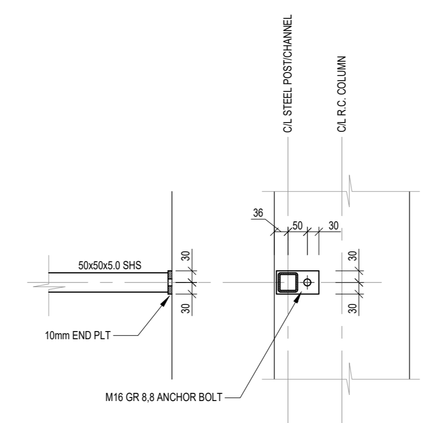
STEEL CHANNEL TO CONCRETE COLUMN DETAIL
