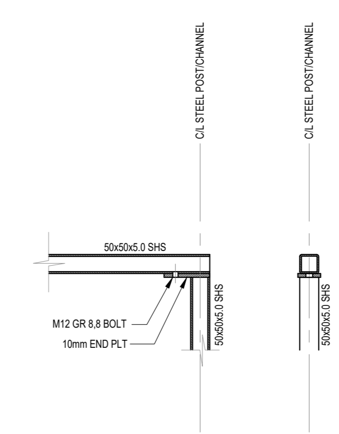
STEEL CHANNEL TO STEEL COLUMN DETAIL
