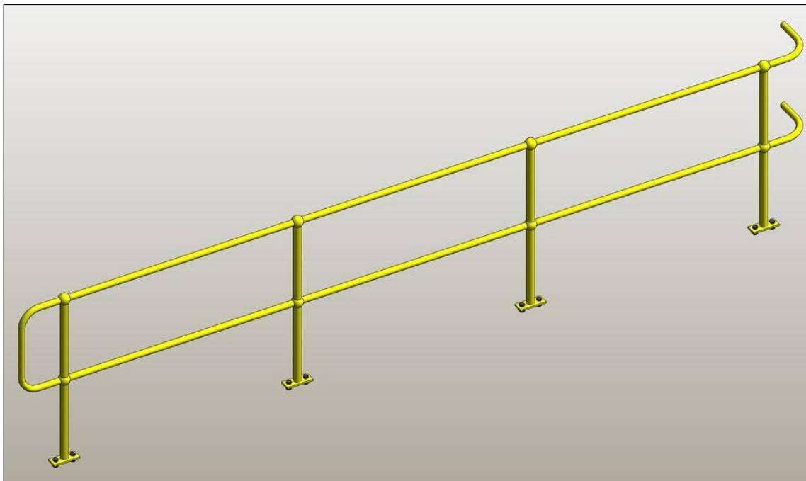
Figure 7: Proposed handrailing
