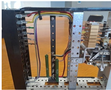
Figure 3 Master Trip Relay
