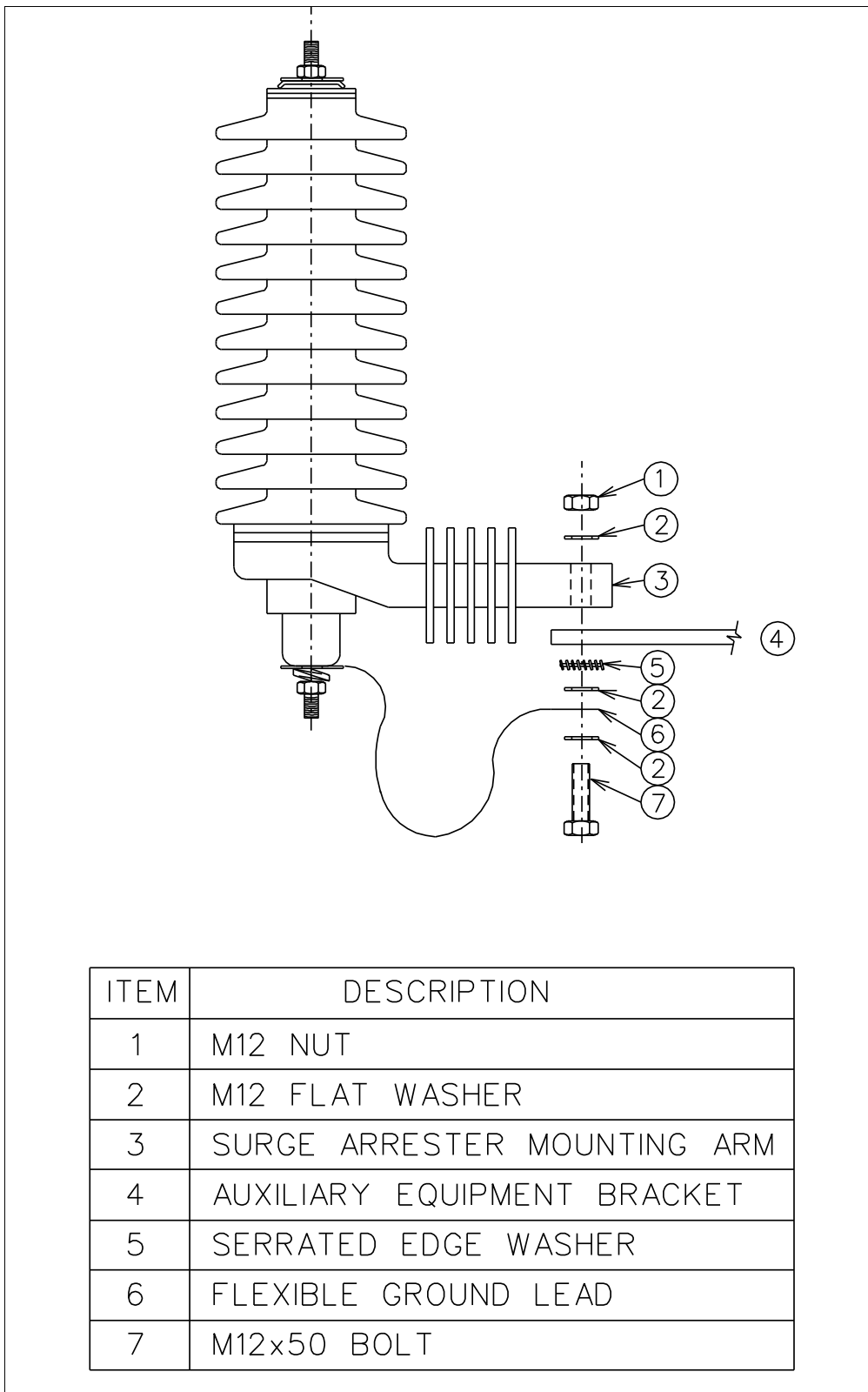
Figure A.4: - Mounting assembly
