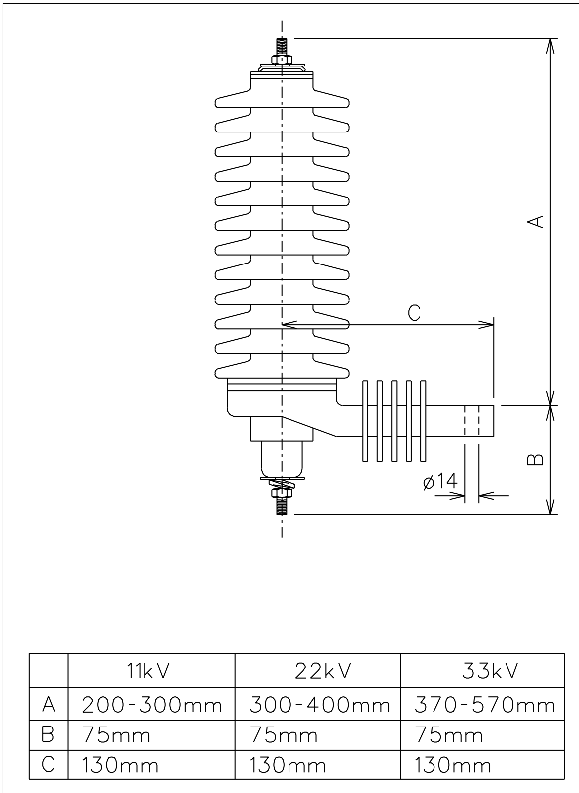
Figure A.1: - Physical dimensions of distribution class arresters
