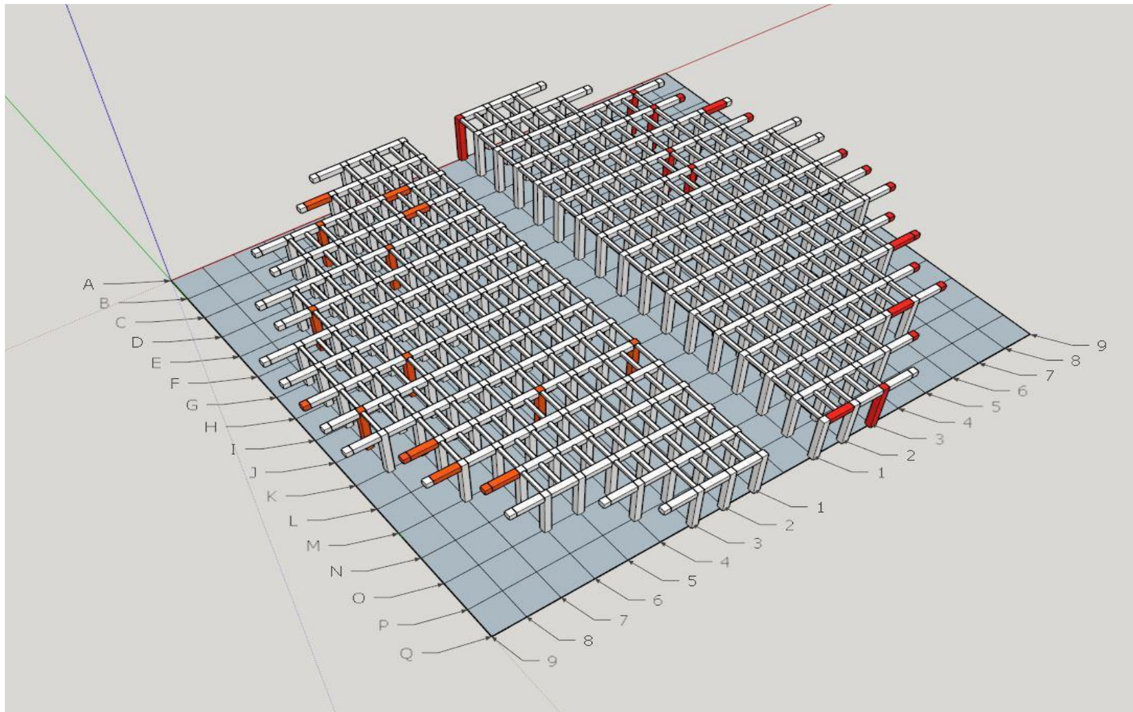
Figure 1: Tower internal arrangement
