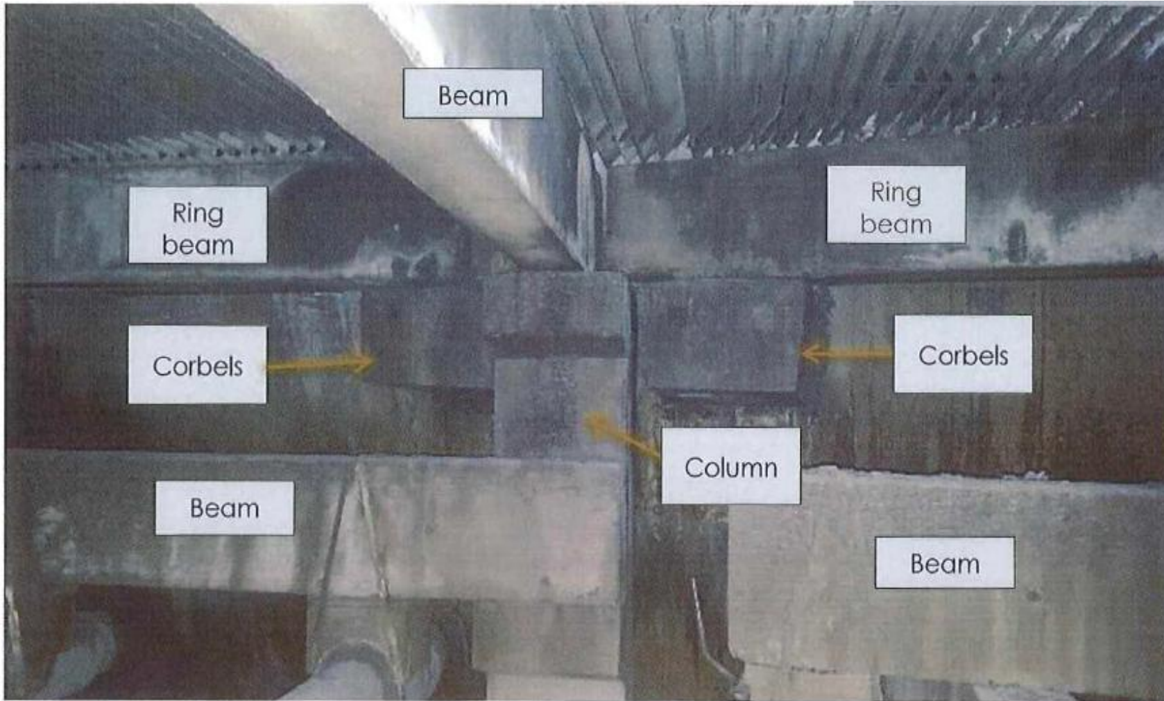
Figure 2: Basic labelling of the Structural components.
