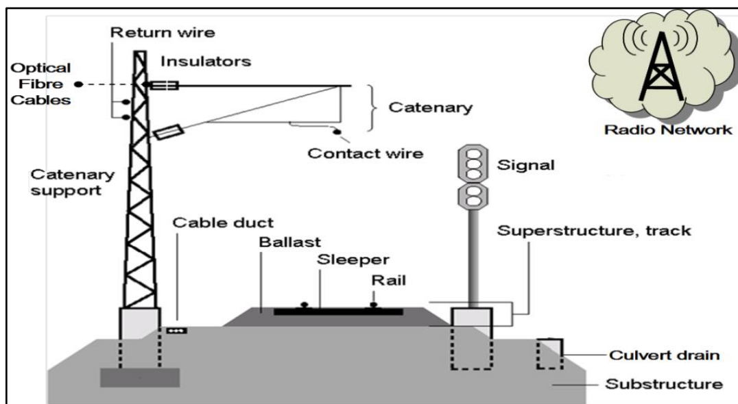
Figure 1: Railway Infrastructure
