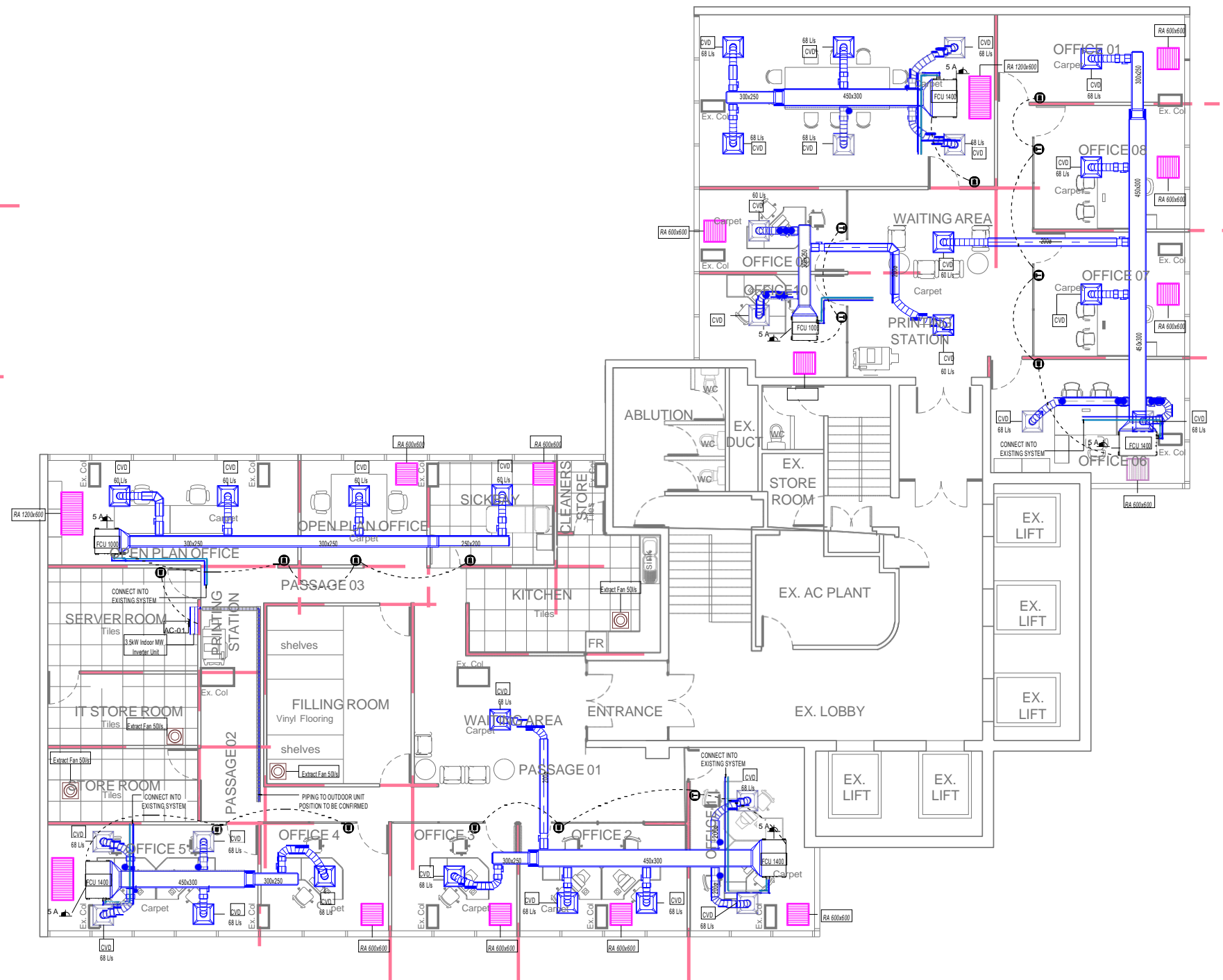
01-SAMSA - SIXTH FLOOR (HVAC)
