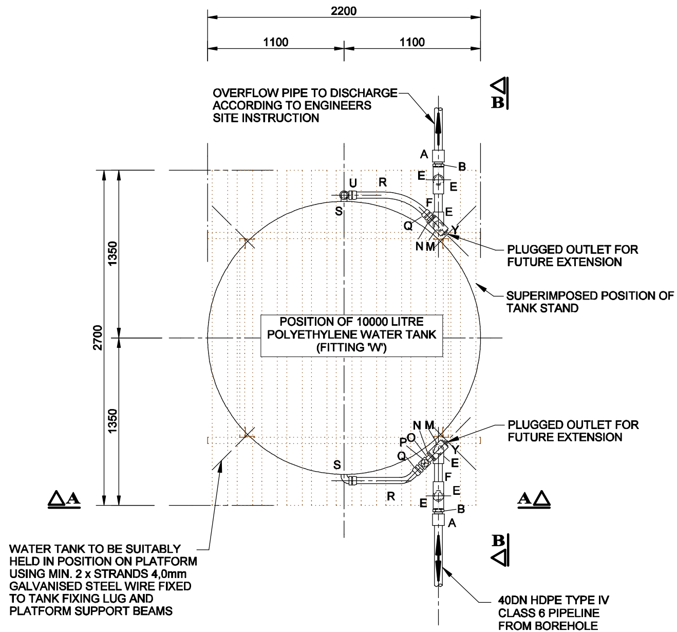
PLAN NTS
