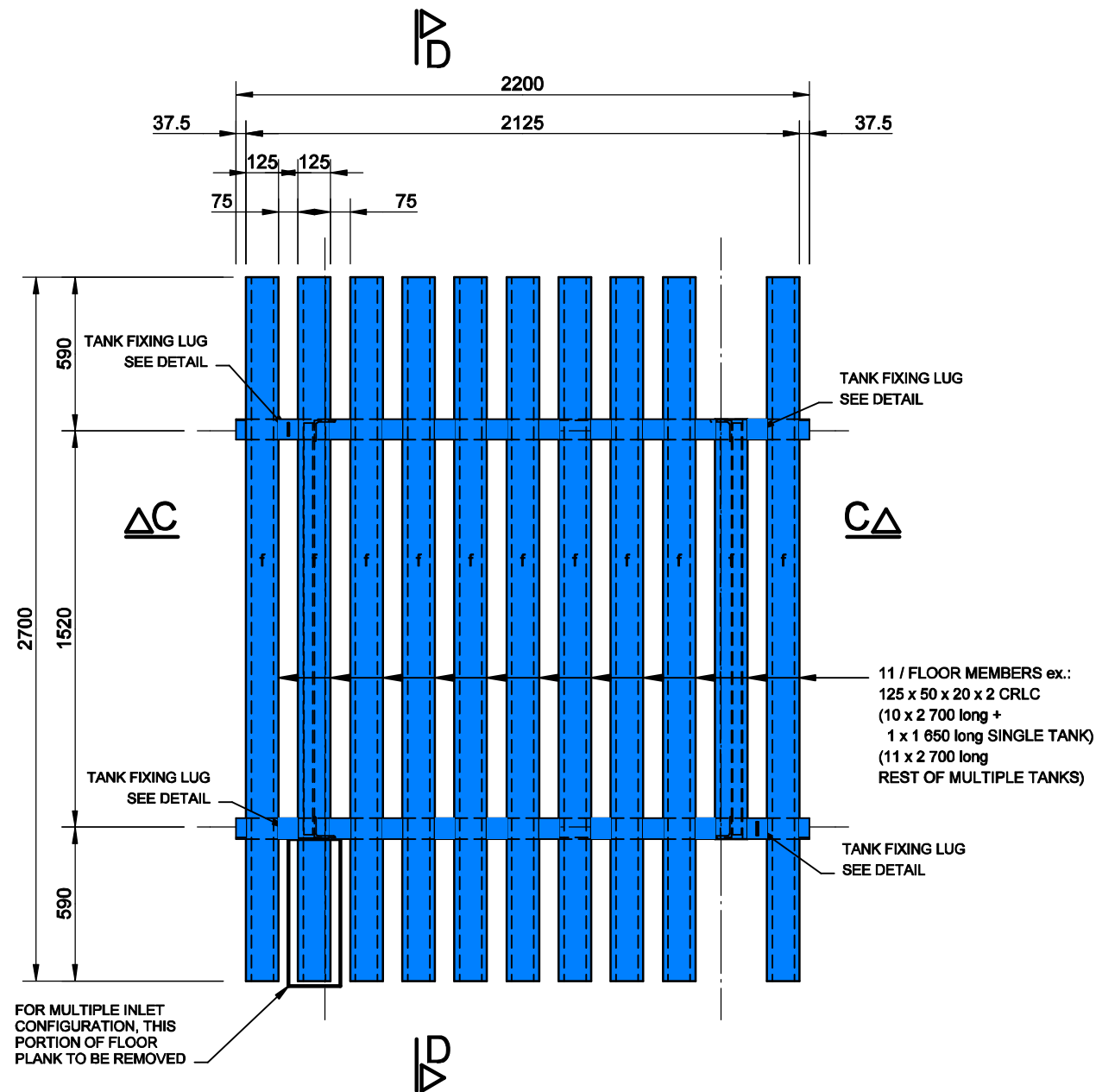
FLOOR LAYOUT 1:25
