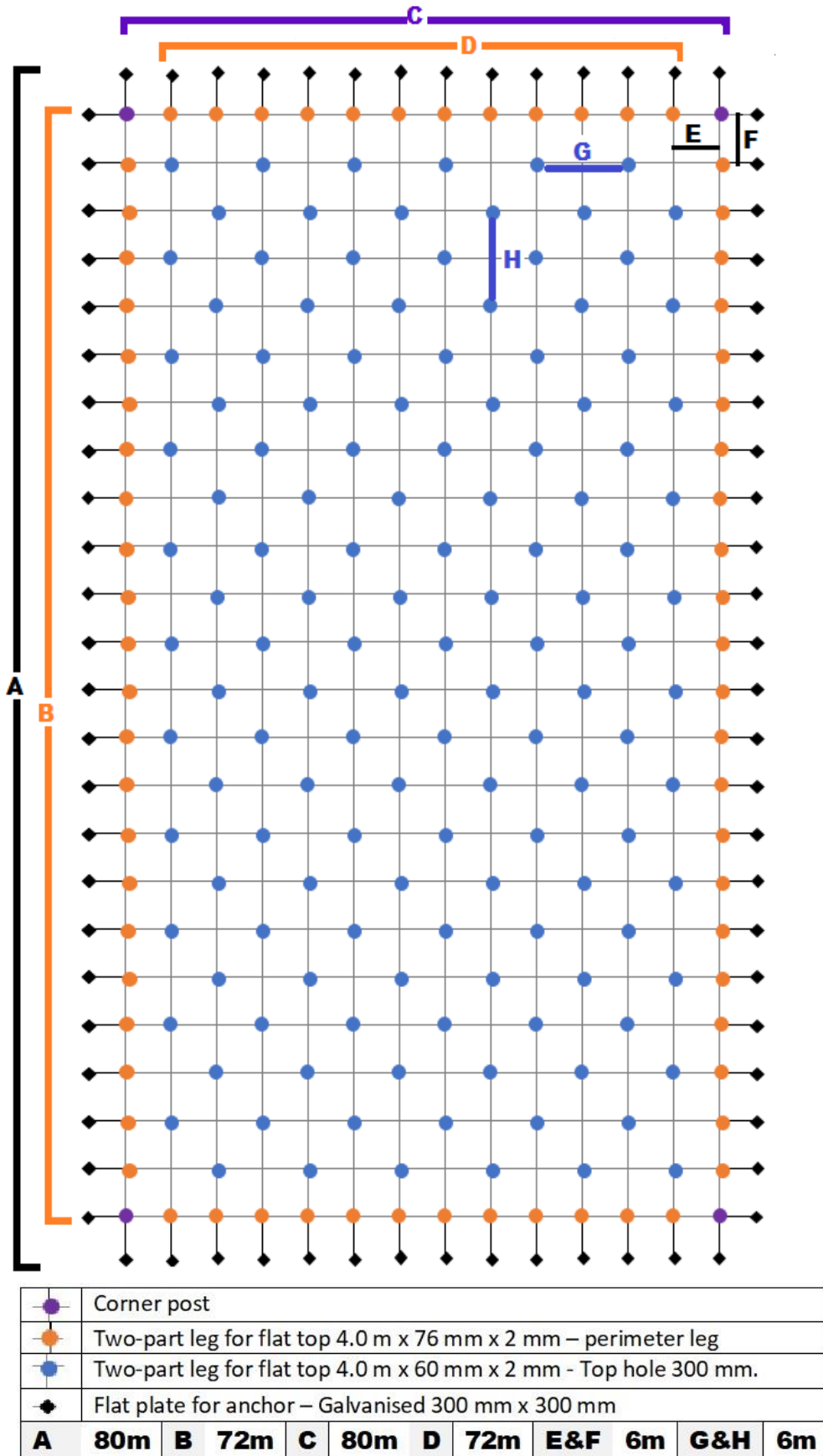
Figure 5: Positioning of poles for full hectare size (Option 1)
