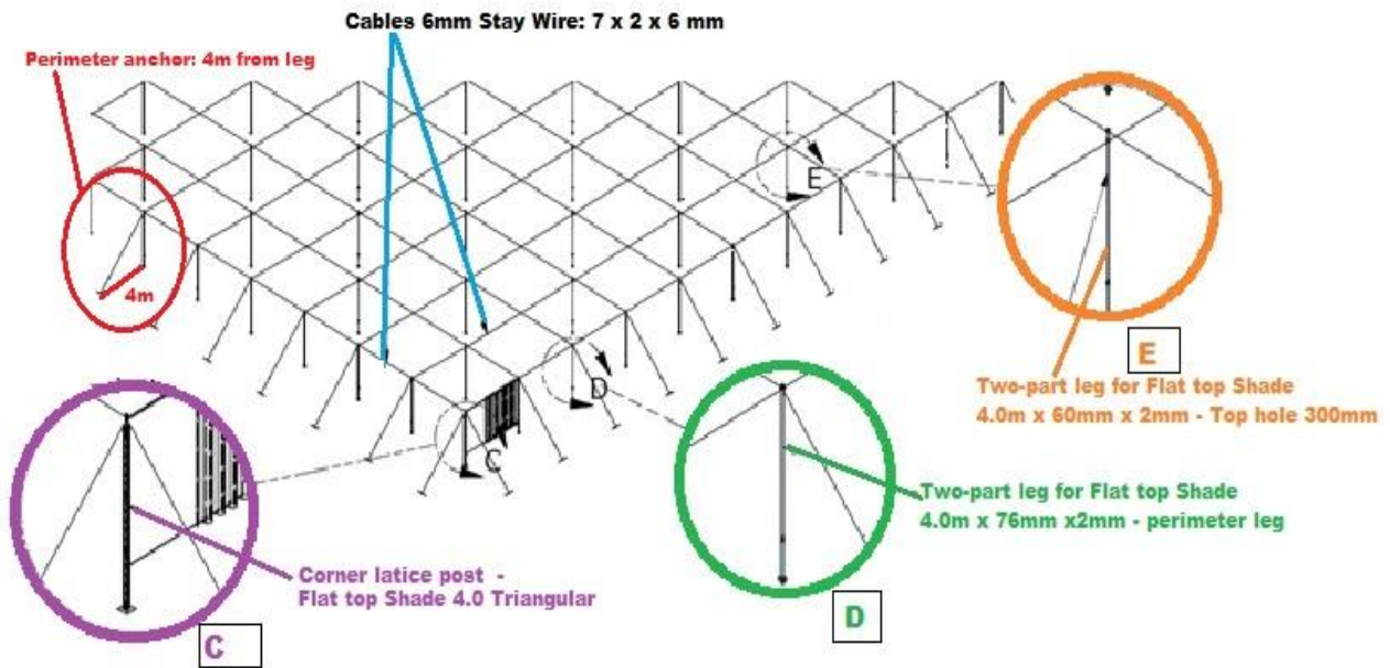
Figure 4: Details of different poles and wires
