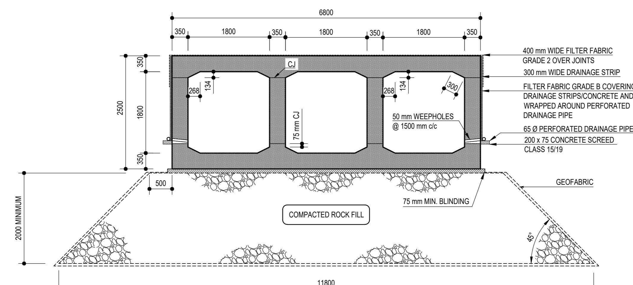
TYPICAL CROSS SECTION 1:50
