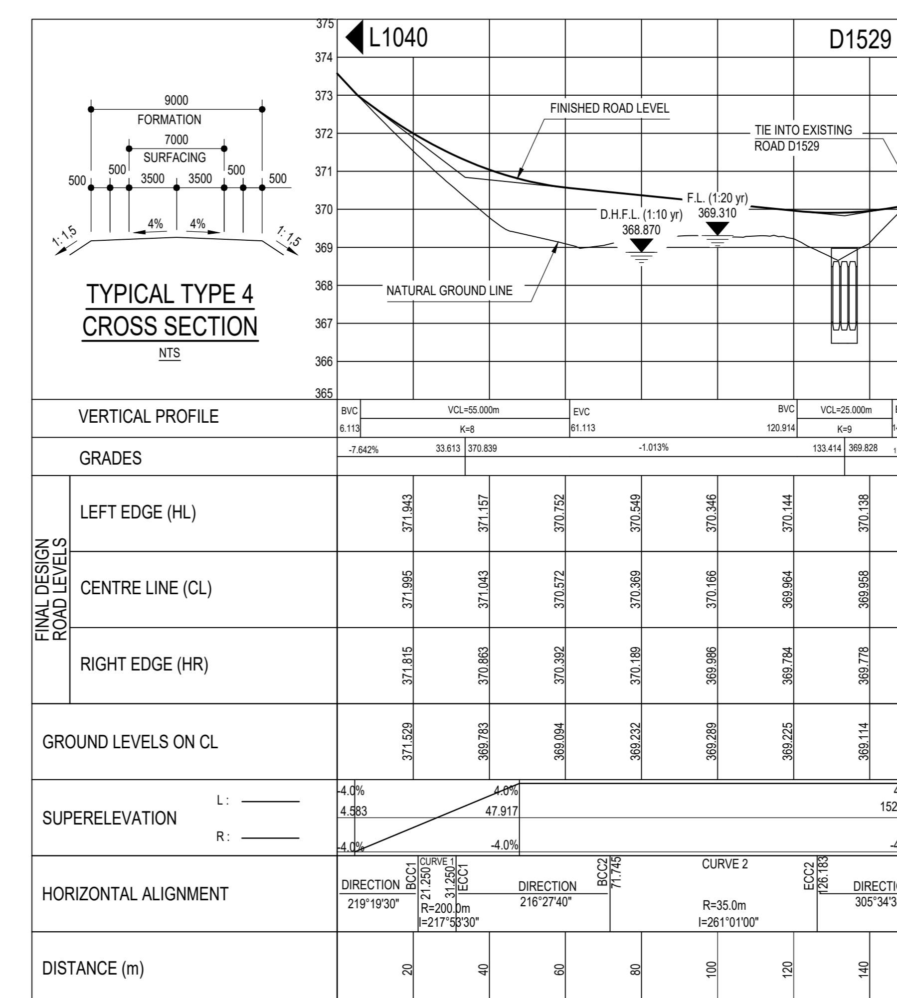
ROAD LONGITUDINAL SECTION HORIZONTAL - 1:1000 VERTICAL - 1:100
