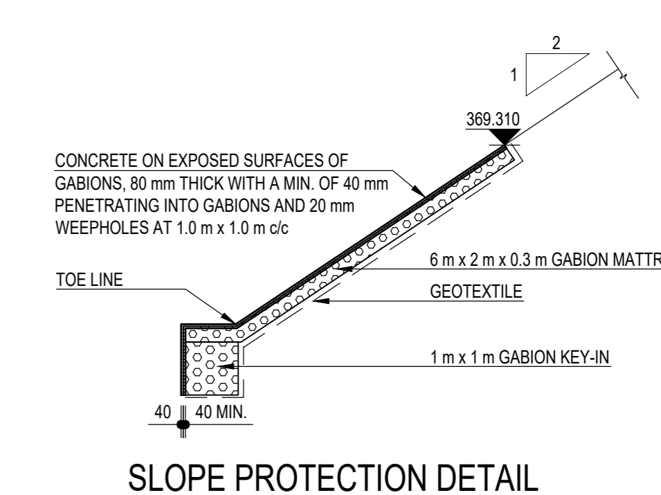
SLOPE PROTECTION DETAIL 1:100
