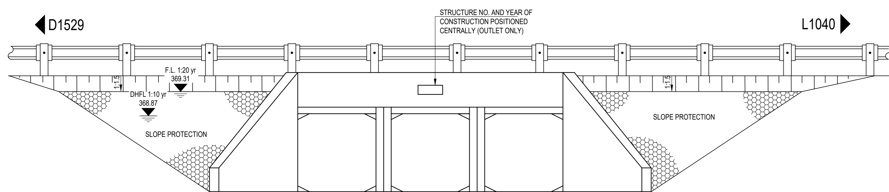
ELEVATION AT INLET 1:50
