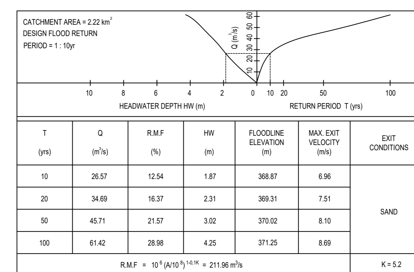
HYDROLOGIC & HYDRAULIC DATA 1:10
